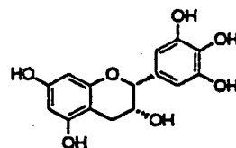
EPIGALLOCATECHIN
